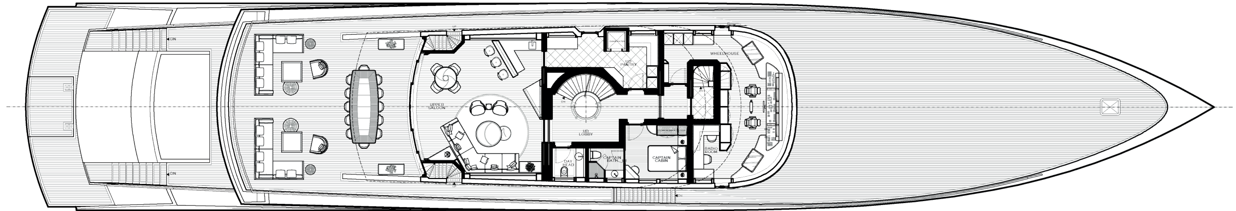
UPPER DECK
